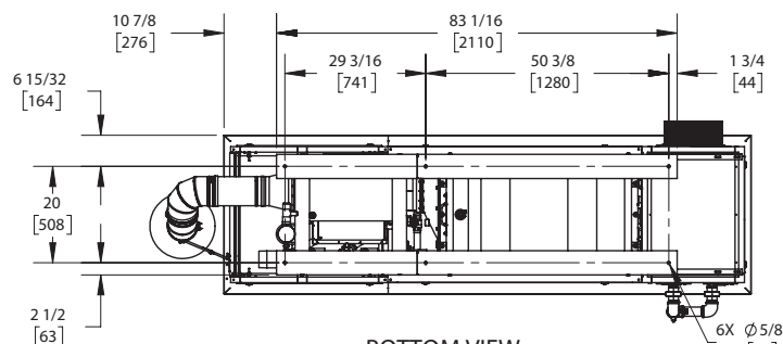
BOTTOM VIEW ASUB-00065_B
